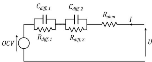
Figure 4: Equivalent circuit model for battery cell
